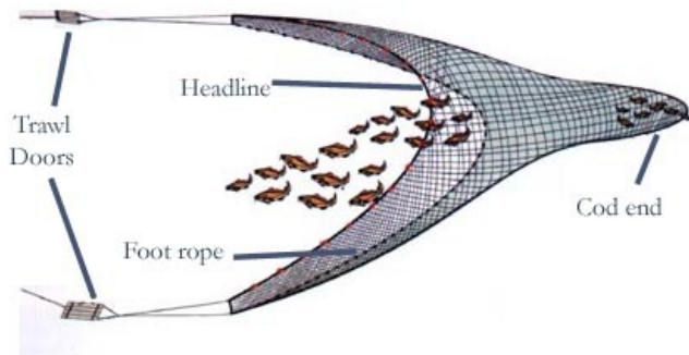
Otter Trawl: A net towed along the seafloor to collect fish and invertebrates.
