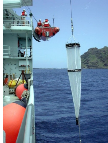
Ring Net: A frame with one net towed through surface water for plankton collection.
